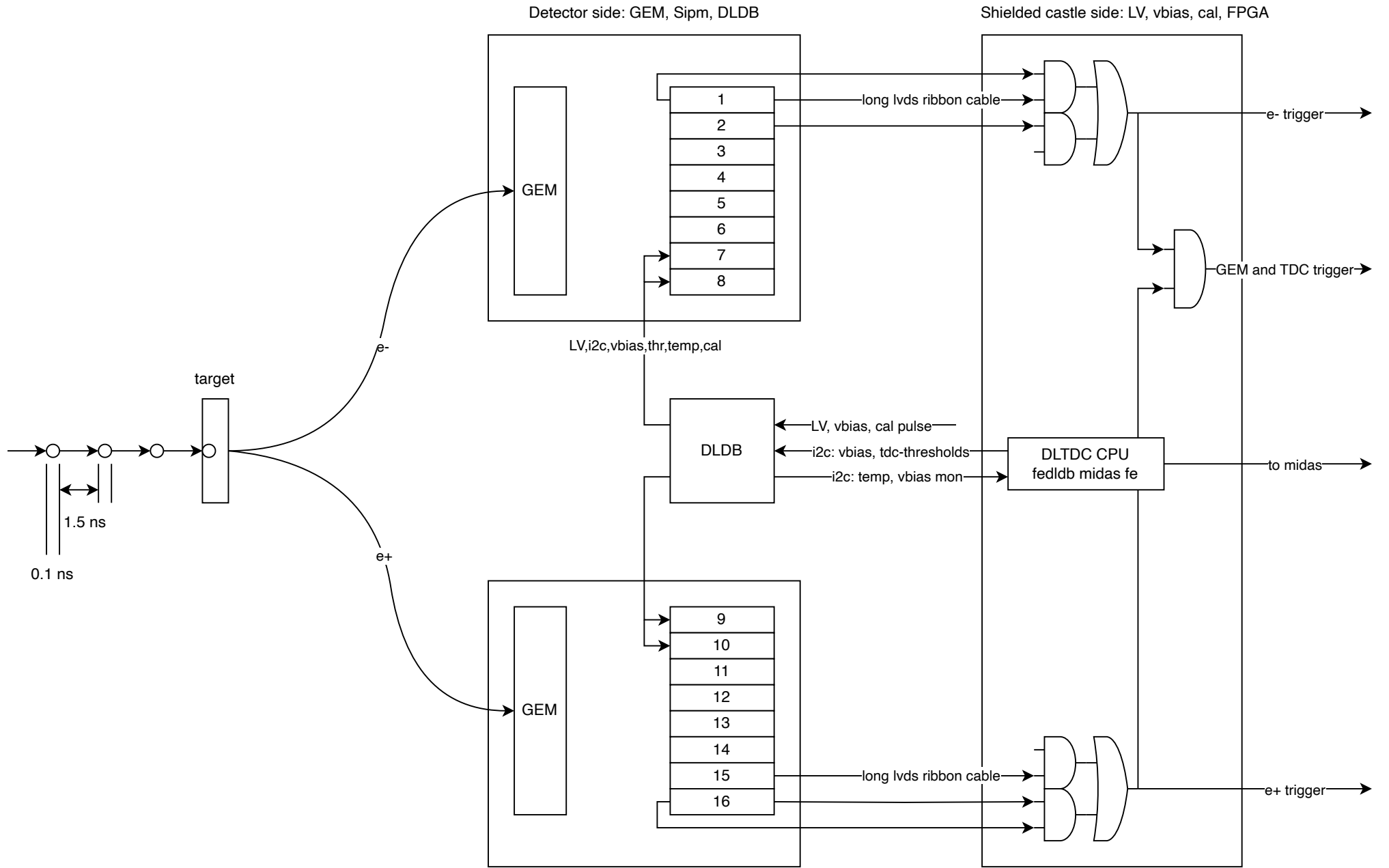
Diagram of trigger logic. KO 8jul2024
