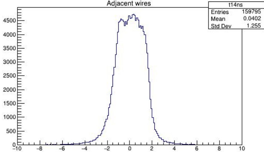
Paddle 1 time difference, t4-t1 (ns) Adjacent wires
