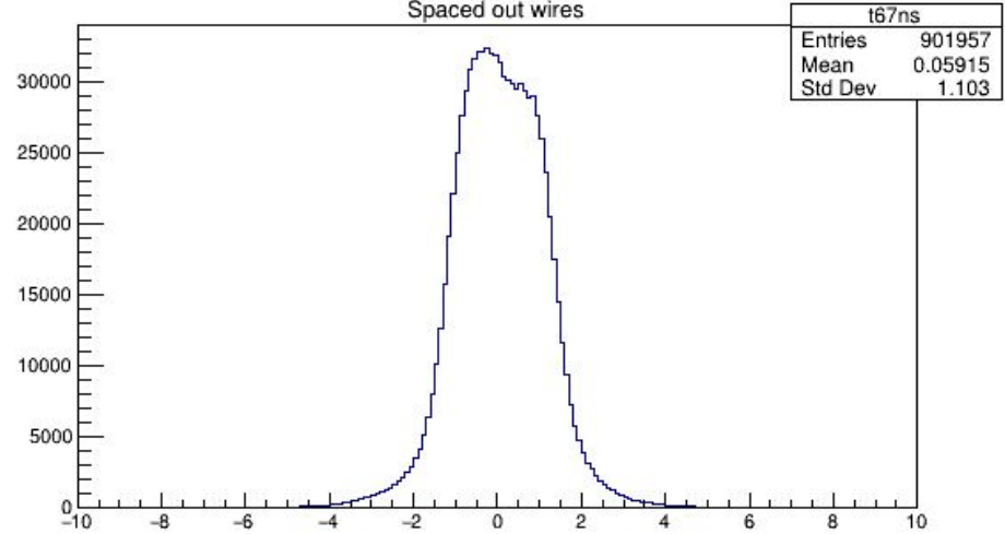
Paddle 4 time difference, t7-t6 (ns) Spaced out wires
