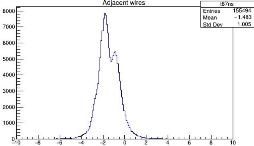
Paddle 4 time difference, t7-t6 (ns) Adjacent wires
